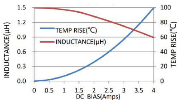
PML2010-1R5-N
