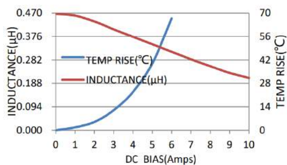
PML2010-R47-N
