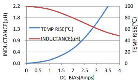
PML2010-2R2-N
