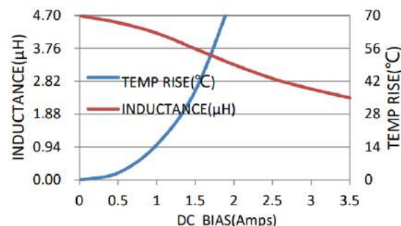
PML2010-4R7-N
